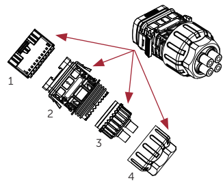
2 Component 1 Housing; 2: Body; 3: Seal part; 4: Nut
