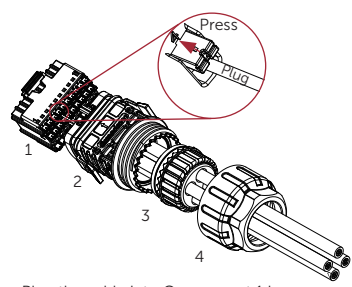
5 Plug the cable into Component 1 in accordance with the following table.
